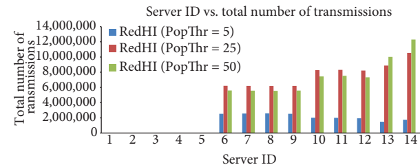
Figure 17. Server ID versus total number of transmissions with arrival rate of 0.2 and popularity threshold values of 5, 25, and 50.
