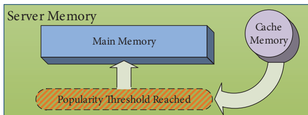
Figure 3. Moving an object from cache to main memory of a server.
