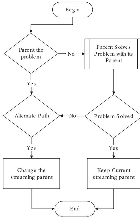
Figure 5. Path change flowchart at a node.
