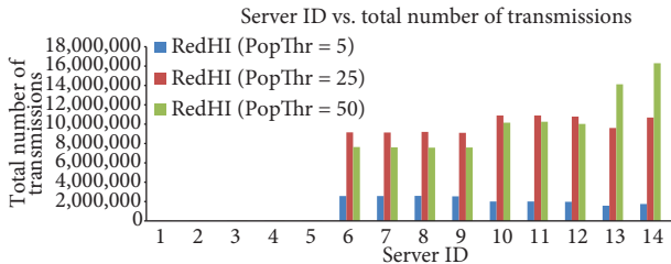
Figure 16. Server ID versus total number of transmissions with arrival rate of 0.15 and popularity threshold values of 5, 25, and 50.
