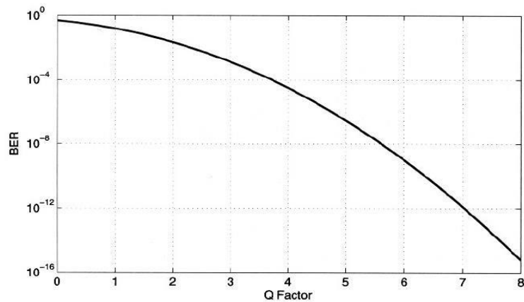
Figure 3.7: BER versus the Q Parament
