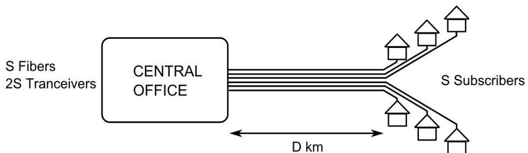
Figure 2.3: Point to Point (P2P) FTTH case
