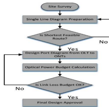
Figure 4.1: GPON FTTH access network design steps
