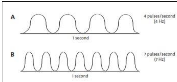
Figure 4.3: Frequency Measurement
