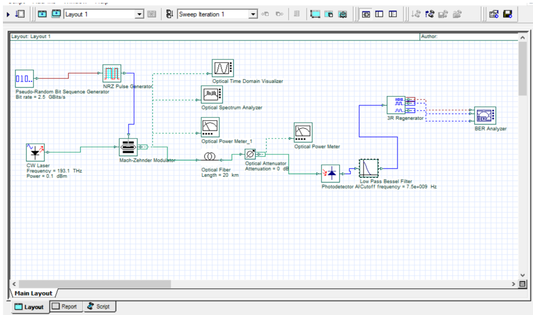
Figure 4.7: Downstream GPON simulation in Opti-system for Single User
