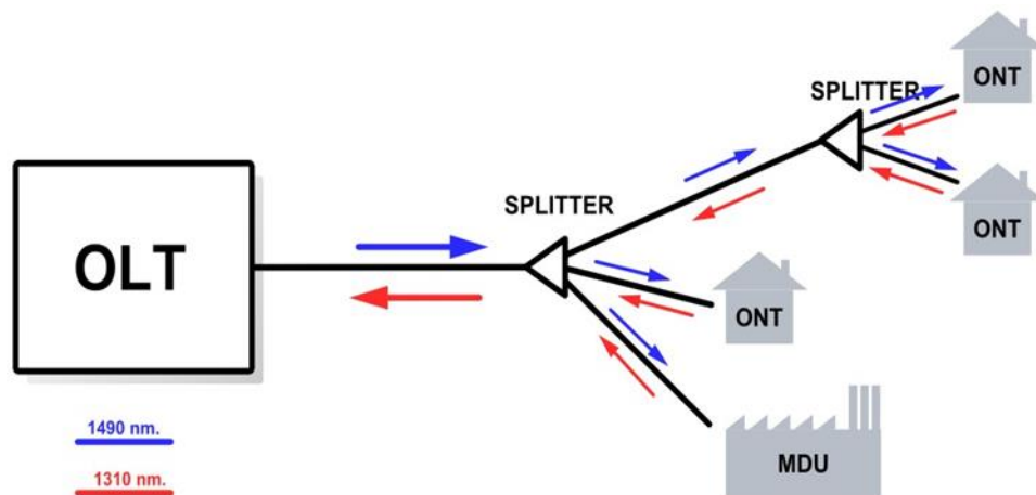
Figure 3.4: Typical GPON architecture
