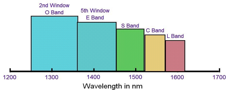
Figure 4.2: Typical optical transmission wave
