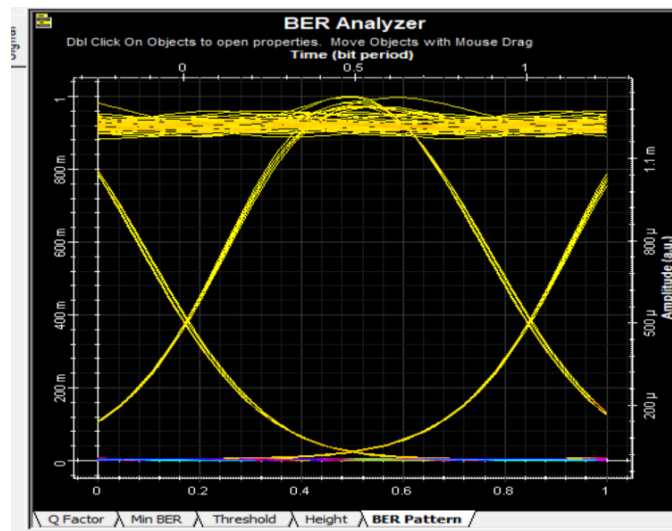
Figure 4.9: Min. BER
