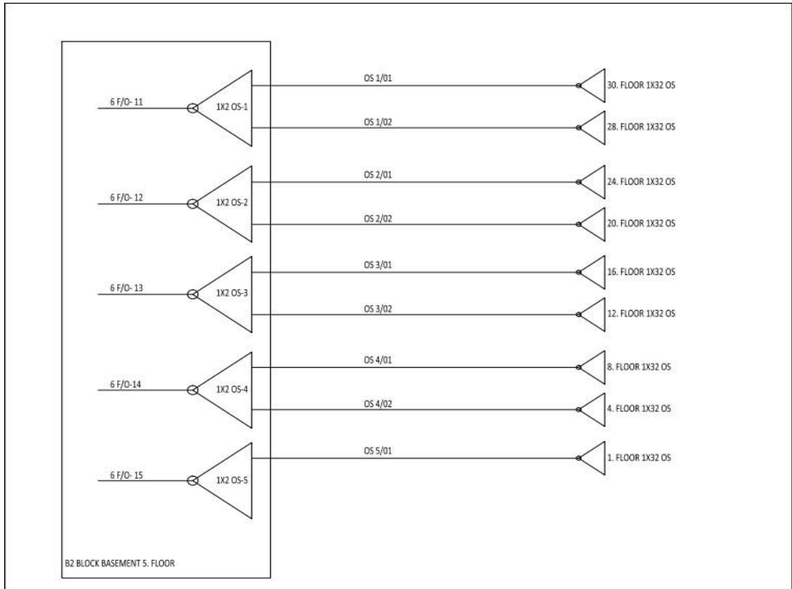
Figure 4.12: B2 blocks Splitter Block Diagram
