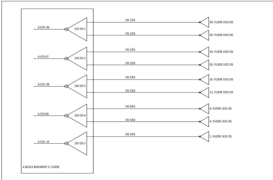
Figure 4.11: A blocks Splitter Block Diagram
