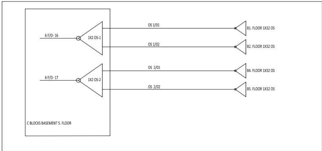
Figure 4.13: C blocks Splitter Block Diagram
