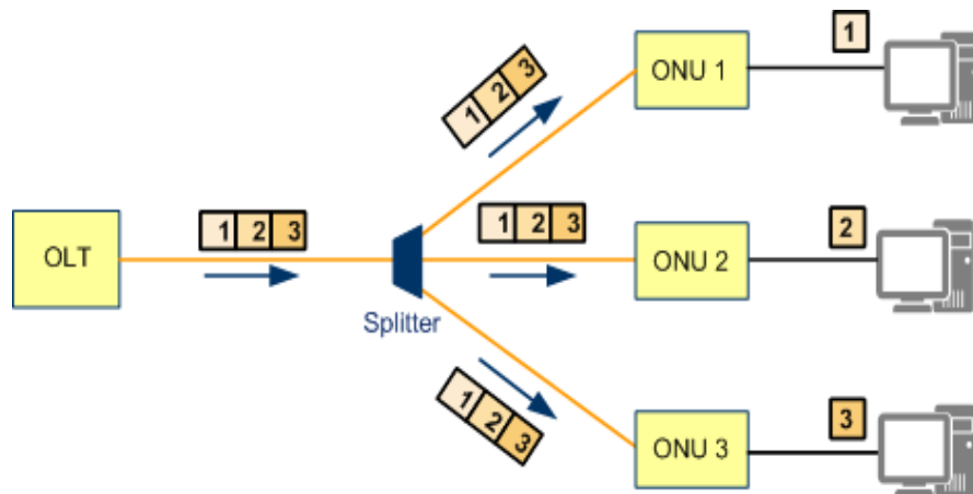
Figure 3.6: traffic in the downstream-direction
