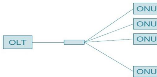
Figure 3.1: Tree with single splitting point
