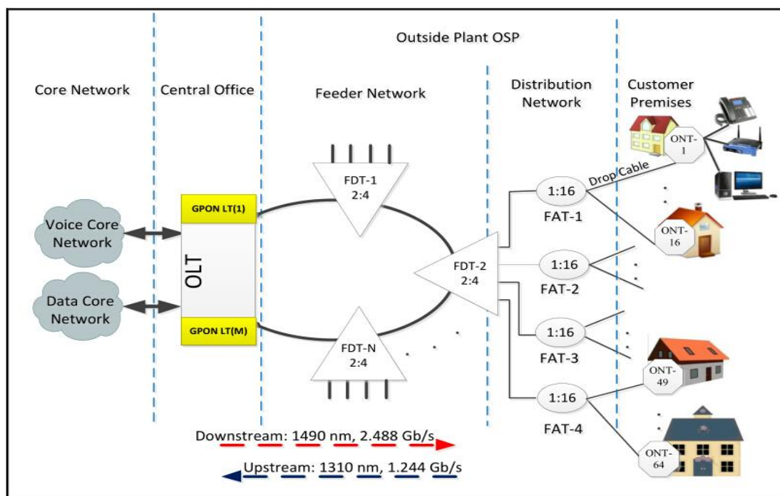
Figure 3.5: Architecture of GPON FTTH Network (Salah Al-Chalabi, 2012)
