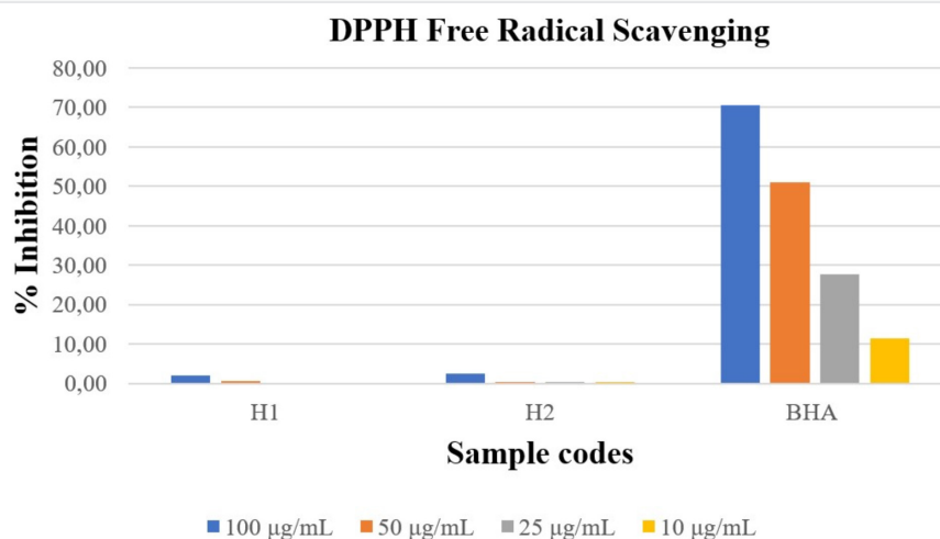
Figure 2. DPPH free radical scavenging activity results DPPH: Diphenyl-2-picrylhydrazyl
